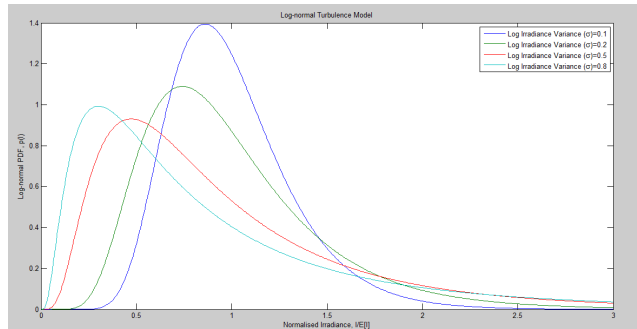
Fig. 4. Log-normal turbulence model
