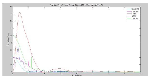
Fig. 3. Comparison of various modulation techniques for optical communication
