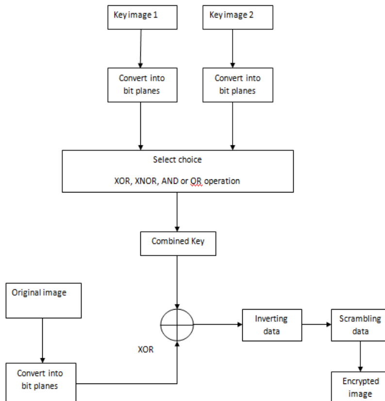
Fig. 3: Proposed CBP scheme with two key images
